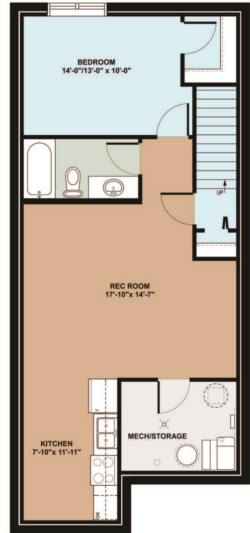
BASEMENT - 691 sq.ft.
