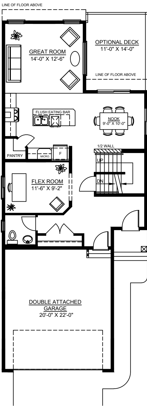
Main Floor 908 Sq Ft
