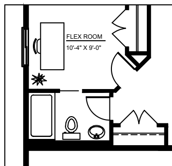
Change Flex Room on Main Level to a 4th Bedroom. Increase % bath to full bath c/w Jack & Jill door
