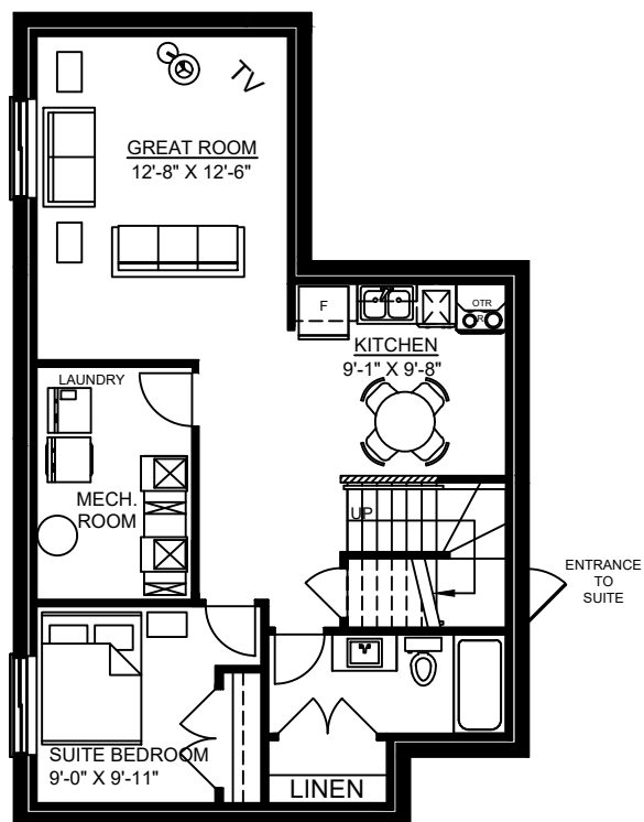
ALT. LEGAL SECONDARY SUITE 722 Sq Ft
