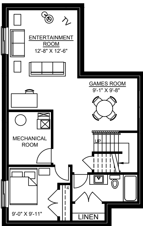
ALT. LOWER LEVEL DEVELOPMENT 738 Sq Ft
