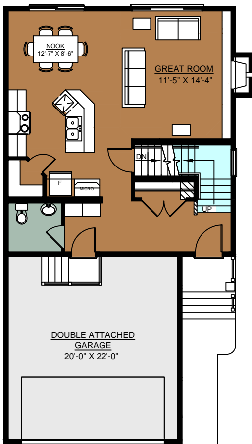
Main Floor 728 Sq Ft
