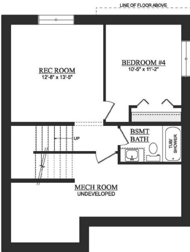
DEVELOPED BASEMENT 452 SQ. FT. (DEVELOPED AREA)
