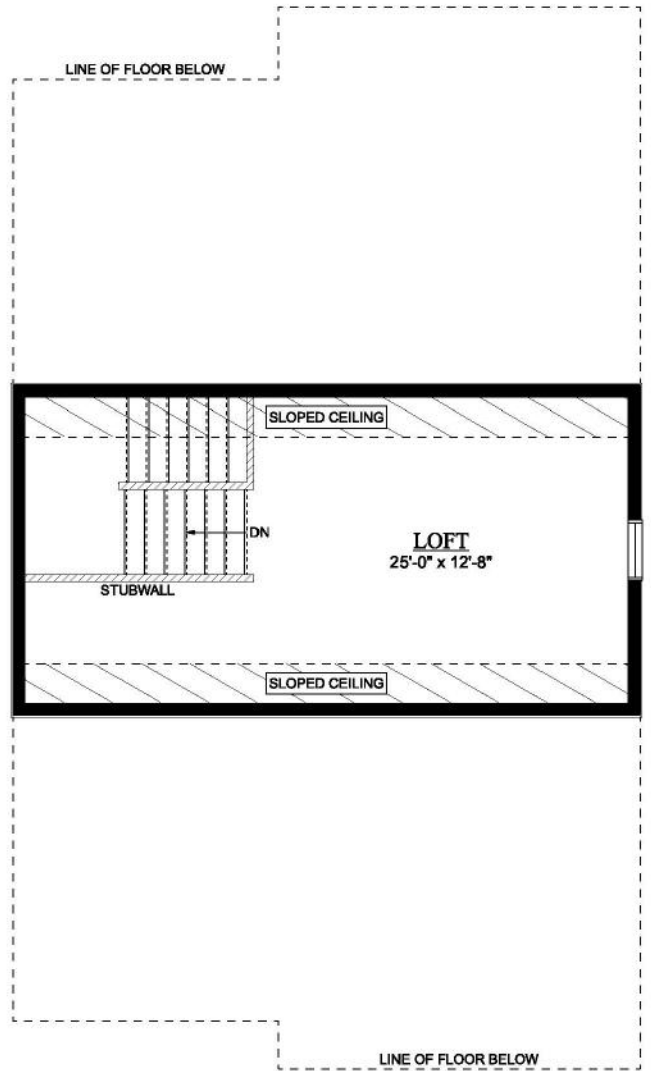
LOFT FLOOR PLAN 355 SQ. FT. (RMS)
