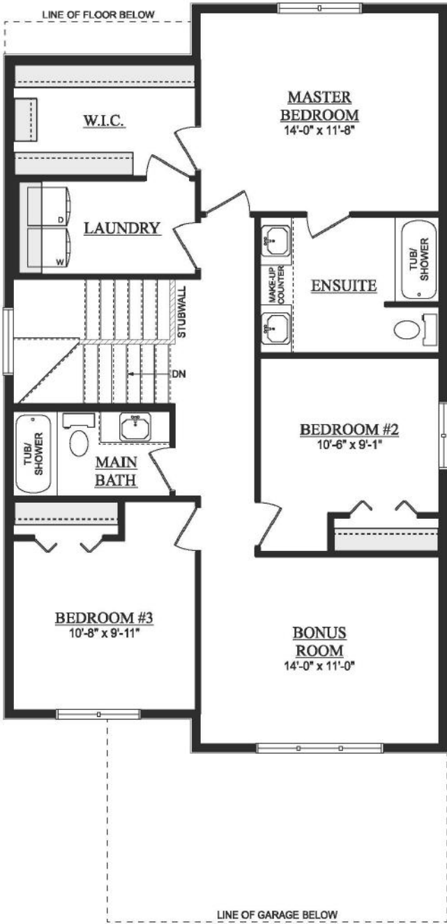
SECOND FLOOR PLAN *OPT. ALTERNATE LAYOUT* 1089 SQ. FT. (RMS)
