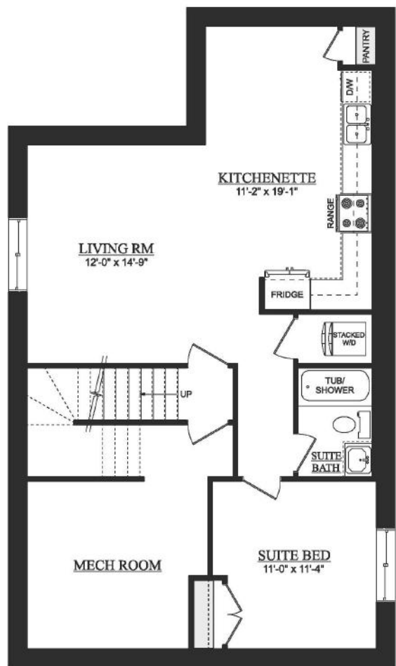
OPT. SECONDARY SUITE 724 SQ. FT. (DEVELOPED AREA)
