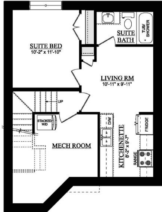
OPT. SECONDARY SUITE 447 SQ. FT. (DEVELOPED AREA)
