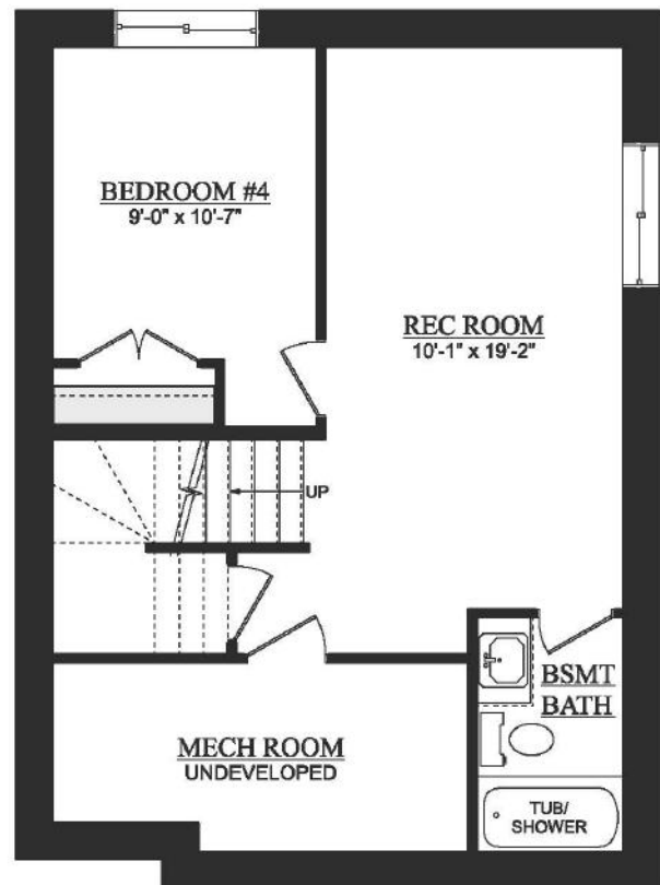
DEVELOPED BASEMENT 438 SQ. FT. (DEVELOPED AREA)
