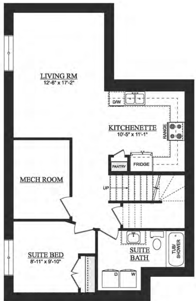
OPT. SECONDARY SUITE 676 SQ. FT. (DEVELOPED AREA)
